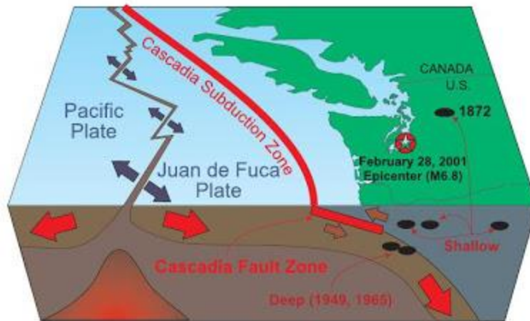
Figure 2: Tectonic features of the Puget Sound Region
